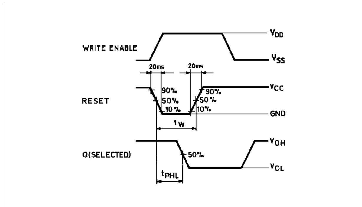
WAVEFORM 4 : MINIMUM PULSE WIDTH ( f=1\text{MHz} ; 50% duty cycle)
